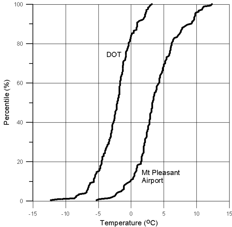
Fig. C1. Percentiles of Mt. Pleasant and DOT temperatures for hours which had vertically-integrated SLW \geq 0.05 mm during the period mid-January to mid-March 1991.
