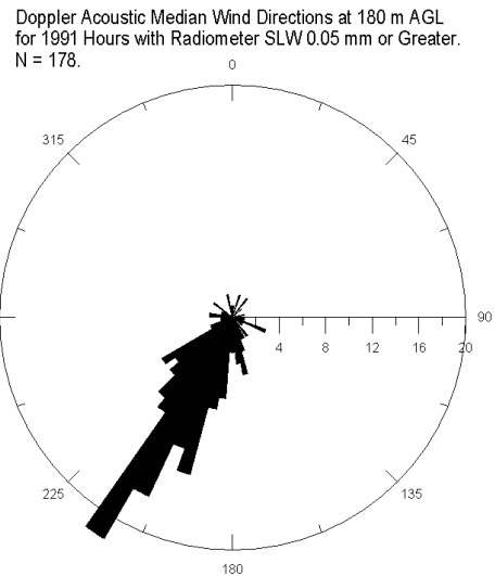
Fig. C2. Wind speeds and directions for Utah Wasatch Plateau investigations in the Sanpete Valley at Mount Pleasant. Plots are for hours in the early 1991 field program which had vertically-integrated radiometer measurements of SLW \geq 0.05 mm. The top two panels are for the surface and the bottom two are for Doppler acoustic wind samples at 591 ft (180 m) agl.
