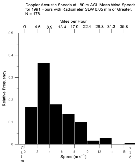
Fig. C2. Wind speeds and directions for Utah Wasatch Plateau investigations in the Sanpete Valley at Mount Pleasant. Plots are for hours in the early 1991 field program which had vertically-integrated radiometer measurements of SLW \geq 0.05 mm. The top two panels are for the surface and the bottom two are for Doppler acoustic wind samples at 591 ft (180 m) agl.
