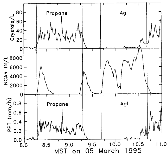
Fig. 1. Temporal distribution of ice crystal concentration (top) and precipitation intensity (bottom), both calculated from the mountain-top observatory 2D-C probe, and acoustical counter measurements of AgI, effective at -20^{\circ}\text{C} (middle panel). Two 3-min "tags" of AgI were released at the beginning and end of the hour of propane release which appear much longer because of the response characteristics of the acoustical counter. The estimated hour of maximum plume presence is shown by vertical lines for propane seeding (left) and AgI seeding (right). The increase in snowfall rate after 10.5 hrs (10:30 a.m.) MST was associated with a natural shower.
